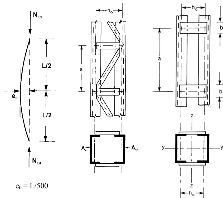
Figure 6.7: Uniform built-up columns with lacings and battenings
